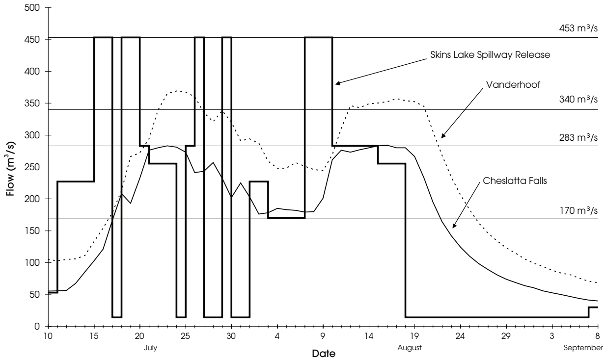
Skins Lake Spillway Releases and Flows in the Nechako River below Cheslatta Falls and at Vanderhoof, July 10 to September 8, 2004
