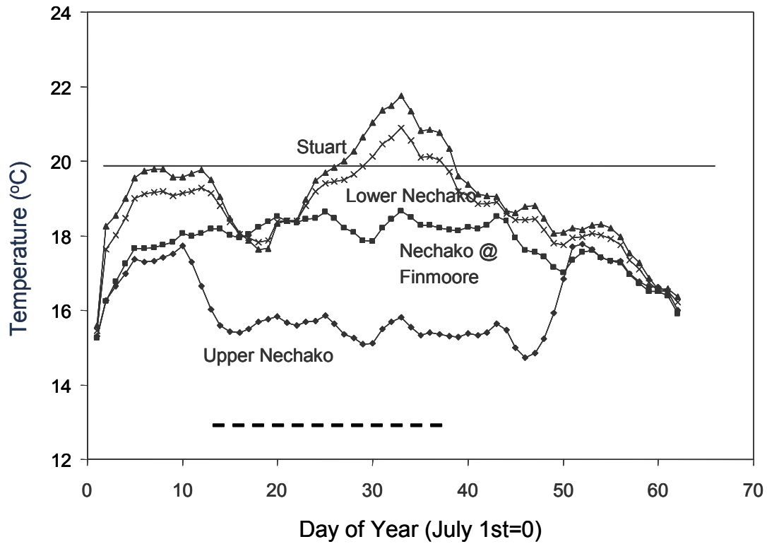
Figure 9: Daily summer water temperature predictions resulting when 53 cms of water (the current pre-operational base release from SLS) is released from Kenney Dam at 10°C. The model uses mean meteorological and tributary conditions during the past 30 years as input. The 20°C temperature target at Finmoore is indicated with a horizontal line. Historically Early Stuart sockeye can enter the Nechako during a period spanning several weeks as described by a dashed horizontal line above the x-axis (Table 1).
