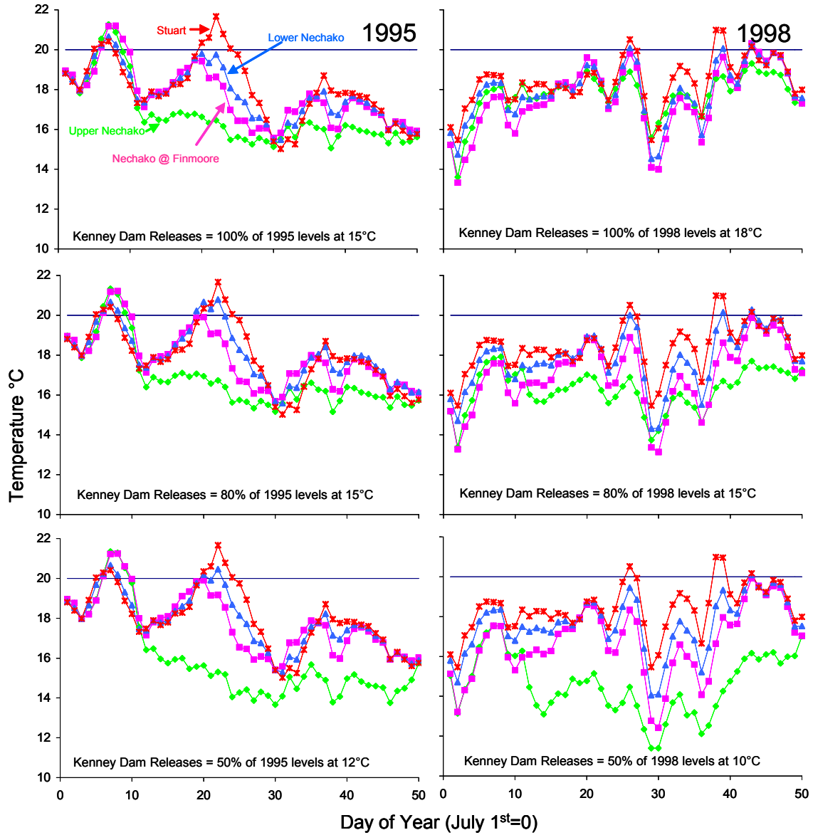
Figure 8: Daily summer water temperature predictions (beginning July 1 st ) resulting from the modelling of various indicated Kenney Dam release volume and release temperature scenarios, at four locations in the Nechako/Stuart watershed. Release volume was based on a percentage of the actual volumes released from the Skins spillway during warm (1998) and cool (1995) years. A horizontal 20°C line identifies the STMP target temperature at Finmoore and a value that approaches the biological limit for migrating salmon. The top left and right graphs are approximate representations of the actual conditions in 1995 and 1998 respectively.
