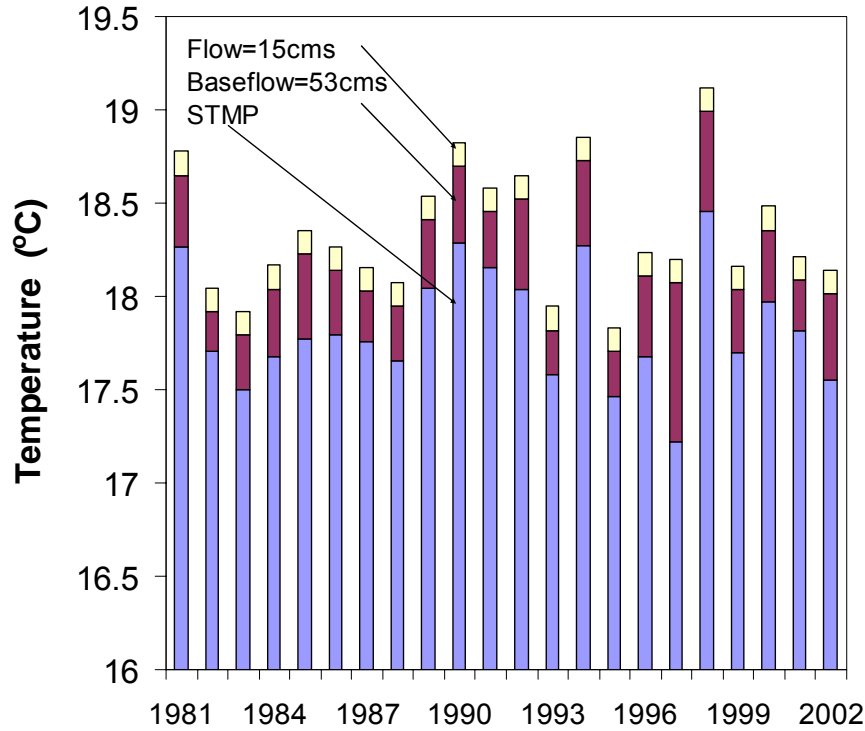
Figure 6: Predictions of mean annual water temperature ( ^{\circ}\text{C} ) at Finmoore in July and August from 1981 to 2002 using the regression model described in Table 5. Three Finmoore flows scenarios were considered; actual STMP flows, the actual spring base release used before the initiation of the STMP (53 cms) and the minimum SLS release during the STMP (15 cms). Flow calculations at Finmoore were modified based on a 4D lag in water release from Skins spillway.
