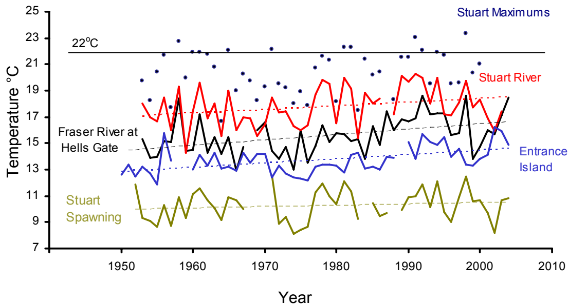
Figure 4: Annual mean temperatures ( ^{\circ}\text{C} ) experienced by the Early Stuart sockeye since the early 1950's during their return from the open Pacific Ocean to their spawning grounds north of Stuart River (Fig. 1). Entrance Island is in the Strait of Georgia 30 km. from the mouth of the Fraser River. Hells Gate is a high gradient reach of the Fraser River approximately 200 km upstream from the river mouth. Stuart River mean temperatures are graphed with annual daily maximum temperatures indicated by individual dots. Data sources are provided in Table 2.
